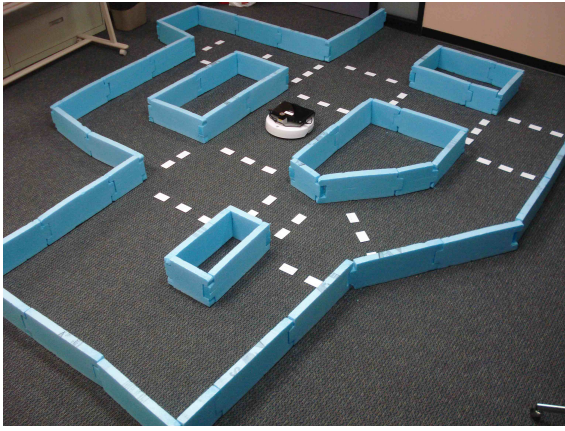
Fig. 1. Robotic InDoor Environment (RIDE). Left: An iCreate mobile platform equipped with a laptop, a laser range finder, and RFID reader moves autonomously through the corridors and intersection of an indoor-like environment, whose topology can be easily reconfigured by moving the foam walls. Right: A robot close-up.
