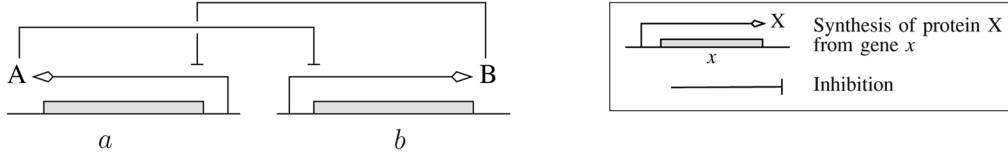
Fig. 1. Cross-inhibition network: gene network comprising two genes a and b and coding for two repressor proteins, A and B. Each protein represses the expression of the other gene, that is, the synthesis of the other protein.
